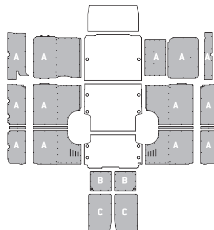
Modelo - Model L5 H3 / XLH3
